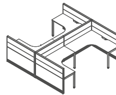
Curvilinear 4-Pax Cluster With Metal Leg C-Shaped
