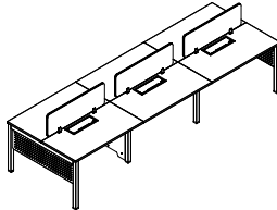
Linear Sharing (Back-to-Back) 6-PAX Cluster with Side Modesty & Straight Metal Legs
