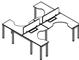
I-Shaped Sharing 2-PAX Cluster with Curvilinear (Deep User Clearance) Worktop
