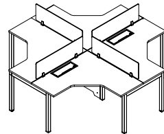
+ Shaped Sharing 2-PAX Cluster with Curvilinear (Chamfered User Clearance) Worktop
